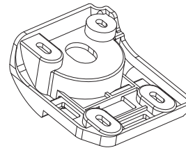
Inner Wheel Housing WHUR045
